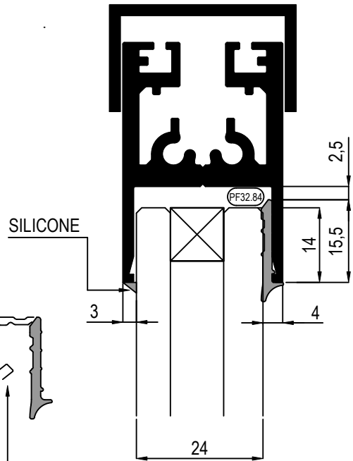
F CAMERA 24mm
